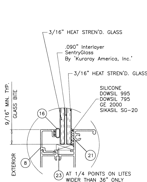
GLASS TYPE 'B' /16" OVERALL LAM. GLASS
